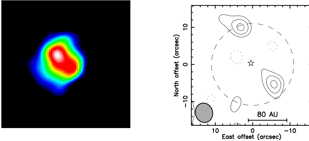
Figure 1. Above we show a SCUBA image of Vega (Holland et al. 1998) and the high resolution PdB image at 1.3 mm from Wilner et al. (2002) focussing in on the central area of the SCUBA image. The high resolution 1.3 mm image resolves the dust emission into two blobs, but with rather low S/N. SOFIA can do much better and the well-known debris disk stars will be prime targets for first light observations.
